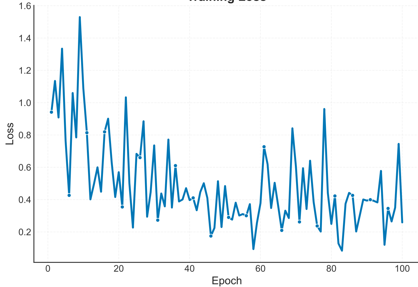
Training Loss
